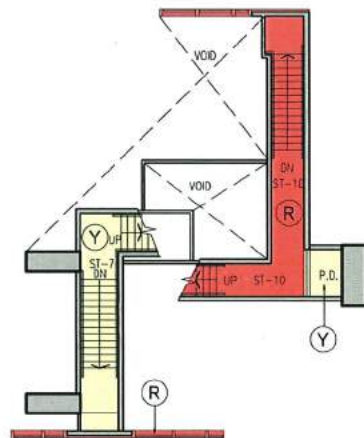
UPPER PART PLAN OF STAIRCASE ST-7, ST-10
