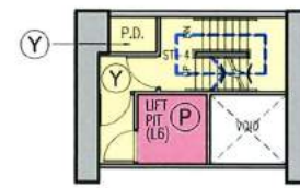
UPPER PART PLAN OF STAIRCASE ST-4
