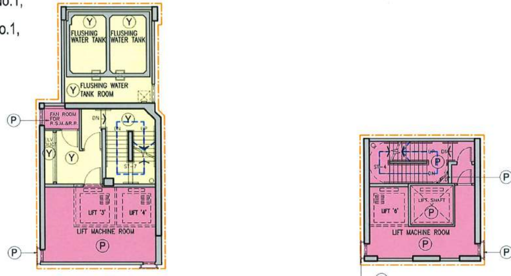
1st UPPER ROOF PLAN
