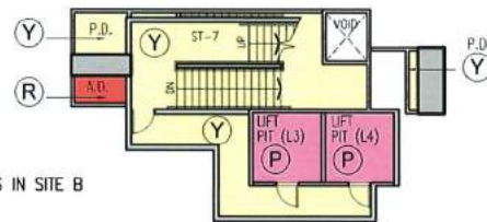
UPPER PART PLAN OF STAIRCASE ST-7
